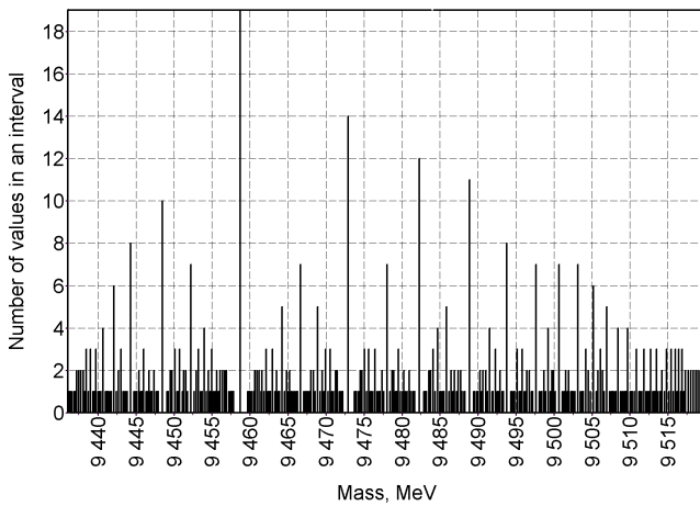
Fig. 19: Mass of the Y (9460) particle in distribution 0.511 e^{x/y} .
