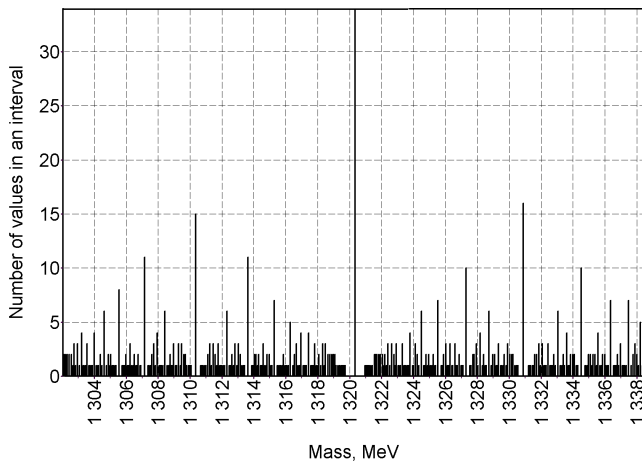
Fig. 7: Mass of the \Xi^- (1321) particle in 0.511 (m_p/m_e)^{x/y} distribution.
