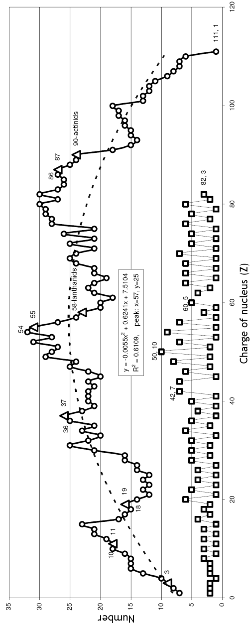
Fig. 4.4: Dependence of total isotopes (circle) and stable elements (square) on atomic number. The triangle designates the beginning of the periods.
