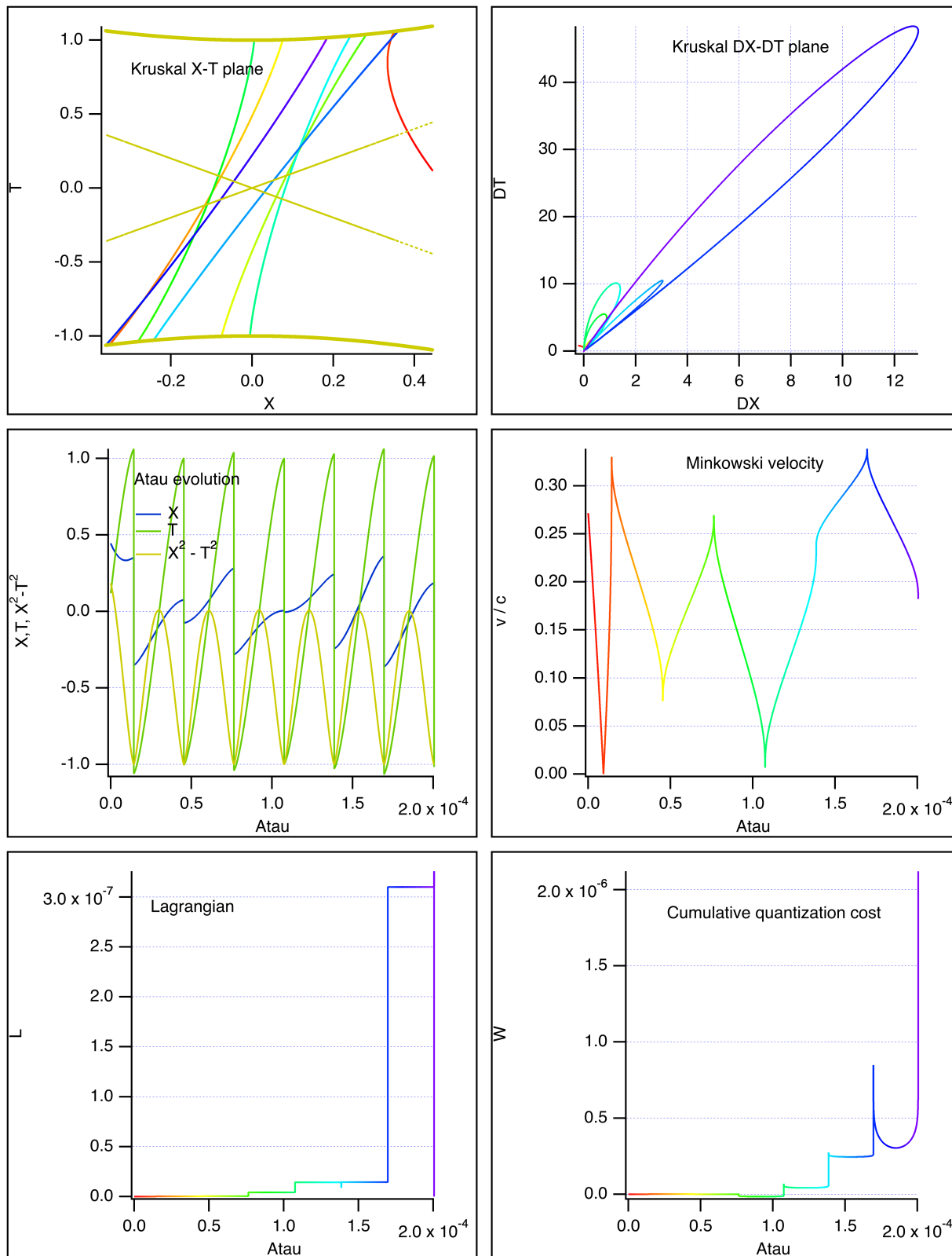
Fig. 5: Trajectory evolving towards the singularity. The variable \text{Atau} is simply the addition of the two real and imaginary clocks. The imaginary time is identified by a negative Lagrangian. The start of the trajectory is in red and its end in dark blue. The passages through the singularity are located at the points where X^2 - T^2 < -1 .
