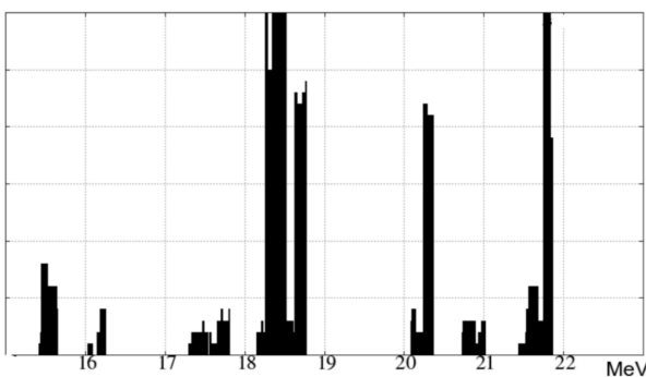
Fig. 6: Calculated spectrum for Al^{27}Si^{28} : A = 27.5 , q = 0.007 , E_{\pi}, E_n(a, b) = 1-27 .
